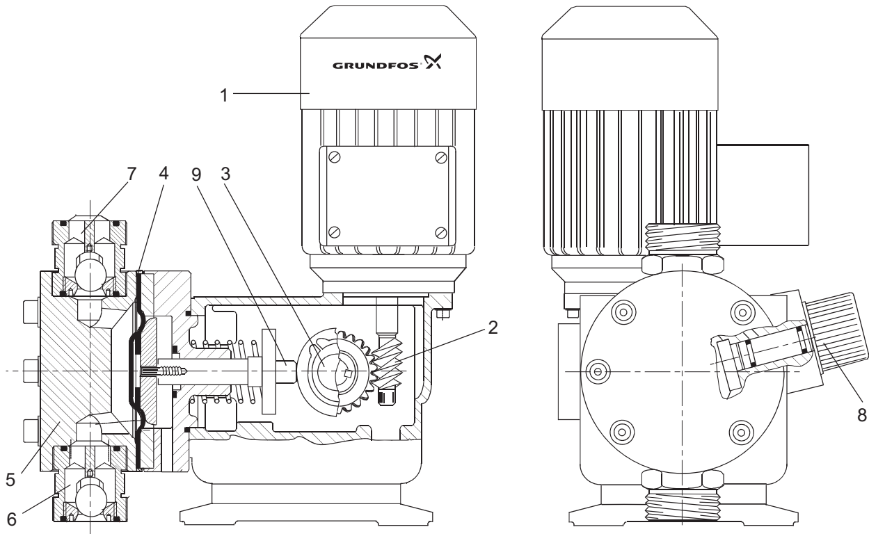
Fig. 23 Sectional drawing, DMX model 226
